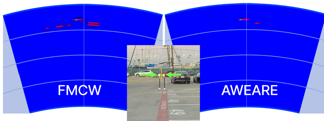
Figure: FMCW radar viewing two adjacent radar targets sees ghosts; AWEARE eliminates these ghosts. Both images were taken with identical hardware at the same filter settings.
